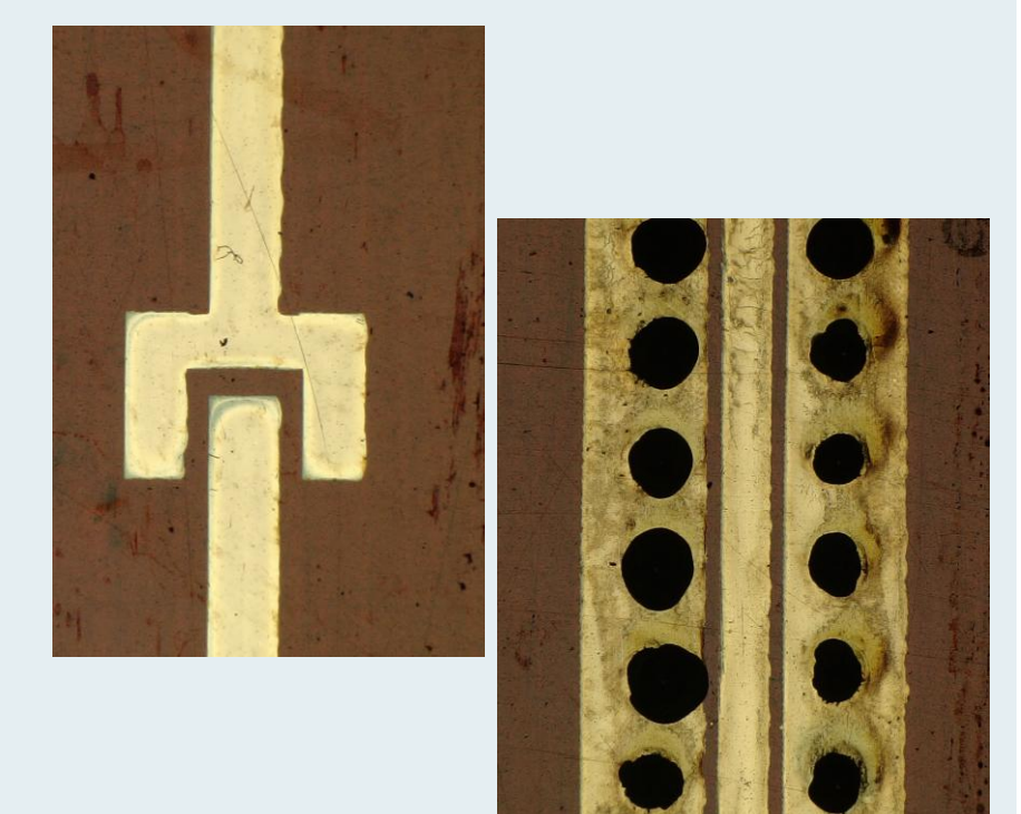
Inkjet-Printed Silver UHF Antenna on a Flexible Substrate
