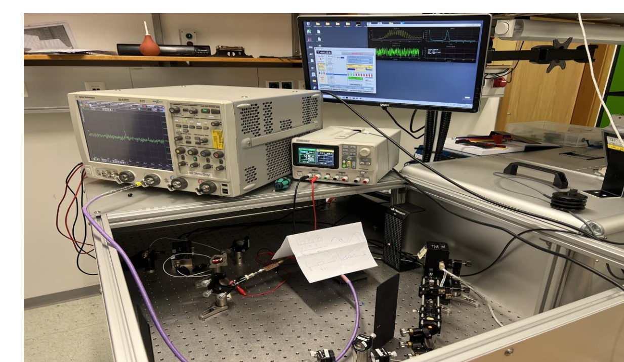
Optically induced switch test setup
